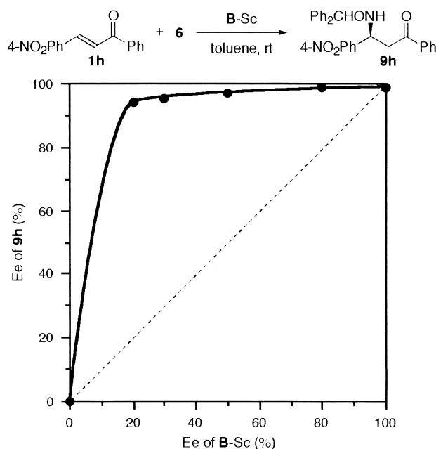
Figure 2. Asymmetric amplification observed in the Sc[( R )-BNP] 3 -catalyzed Michael addition of 6 to 1h .
